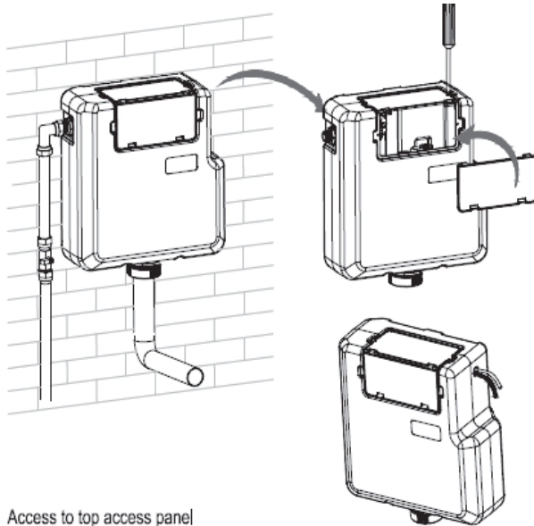
Access to top access panel
